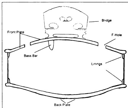
Figure 2. Schematic transaxial section through the middle bout, at the level of the bridge. Note the two “f” holes located between the foot of the bridge and the edge of the front plate. The linings attach the front and back plates to the ribs.
