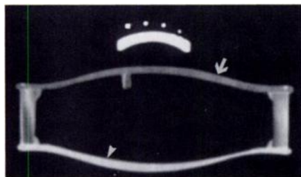
Figure 3, 4. (3) Coronal CT scan of an exquisite violin crafted by Antonio Stradivari demonstrates the rib outline. This outline provides the modern luthier with an exact copy of the edges. Note the round sound post (arrow), a 5.5-mm-diameter spruce rod that establishes a connection between the front and back plates. (4) Transaxial CT scans through the middle bout of (a) a violin crafted by Nicolò Amati in 1654 and (b) an inexpensive German student violin. Note the exquisite archings and changes in thickness of the anterior front plate (arrow) and posterior back plate (arrowhead) of the 1654 Amati violin compared with the front and back plates of the student violin. All the student violins had very thick and poorly arched plates.
