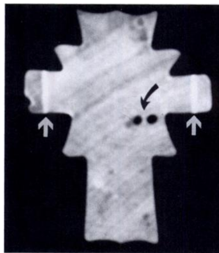
Figure 7. Transaxial CT scan obtained through the scroll of a 1730 Domenico Montagnana cello. Note the hyperattenuating glue lines (straight arrows) from previous repair and wormholes (curved arrow) caused by infestation from the larvae of the beetle, A domesticum .
